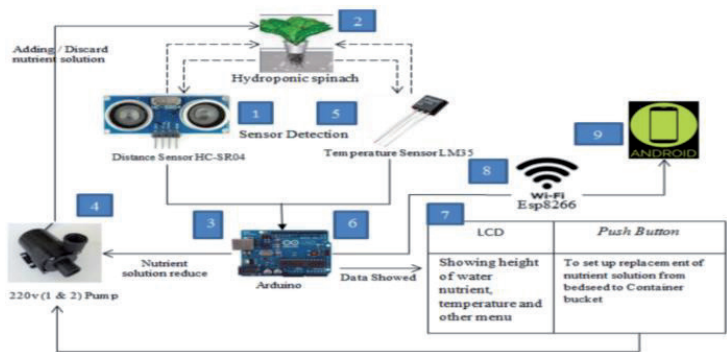
Figure 20. Automated hydroponics nutrition plant system.
