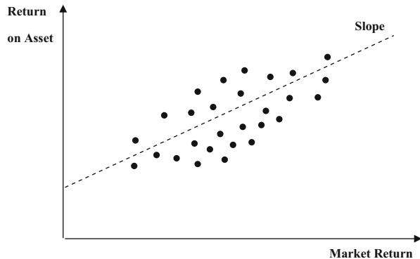
Fig. 8.1 Graph of a linear regression
